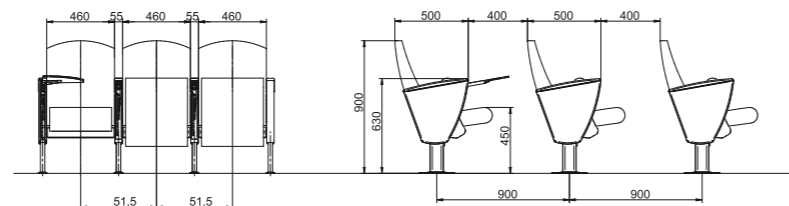
Aura 100 with folding writing tablet
