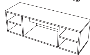
180x50x58h
